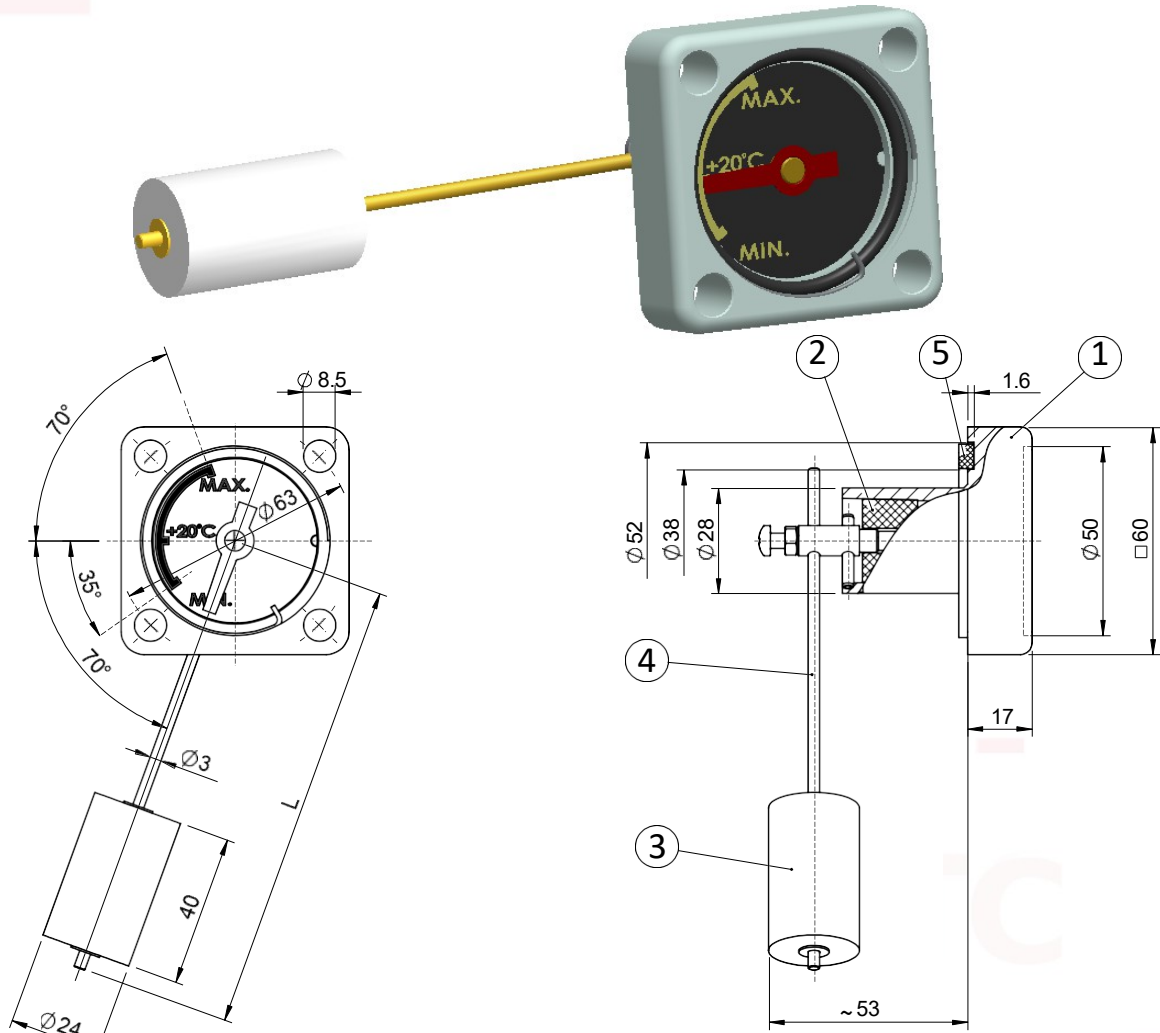
mounting example
