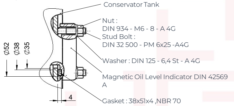
mounting example
