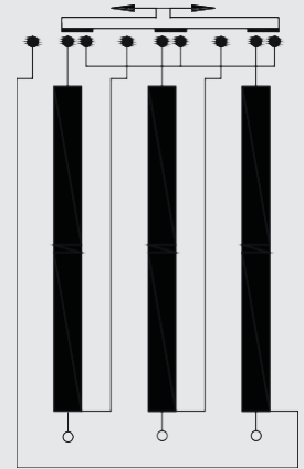
Star - delta coupling
